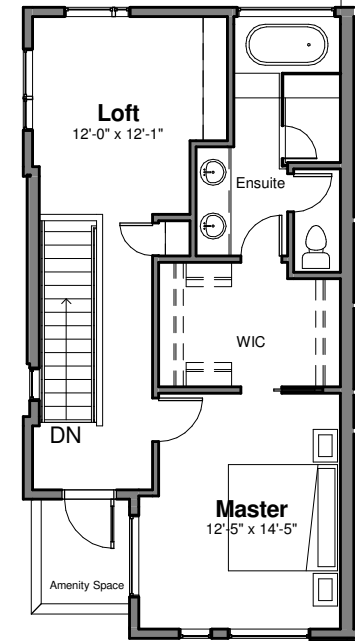
Unit A - Third Floor 659 SF
