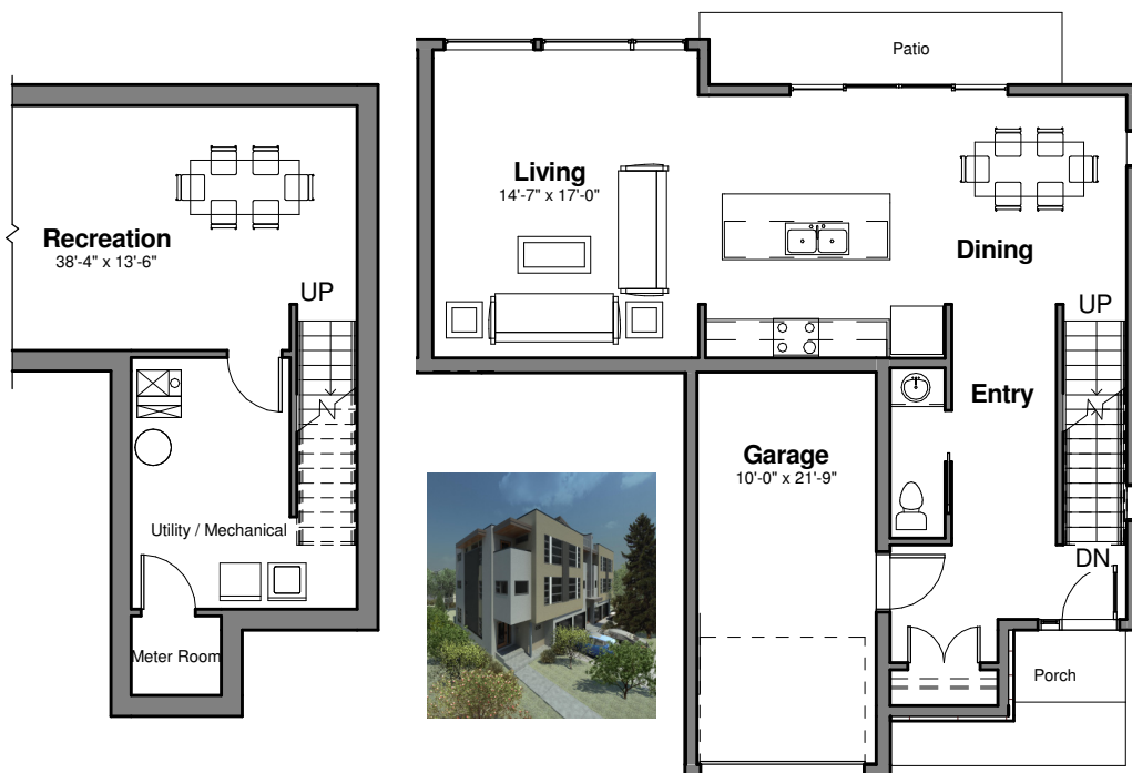
Unit D - Basement (East)
