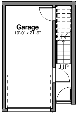
Unit B - Main Floor
