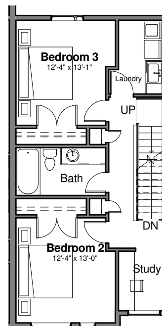
Unit D - Second Floor 702 SF
