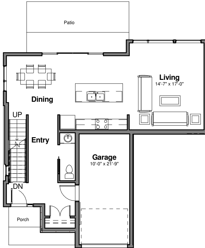
Unit A - Main Floor 888 SF
