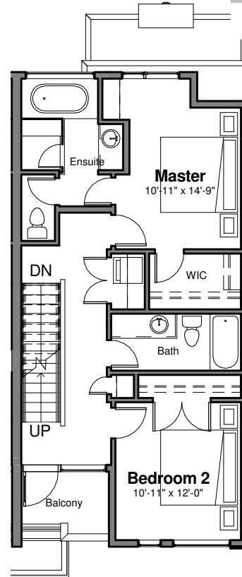
Unit C - Third Floor 710 SF
